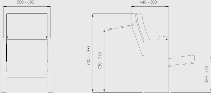
B) cassette version
