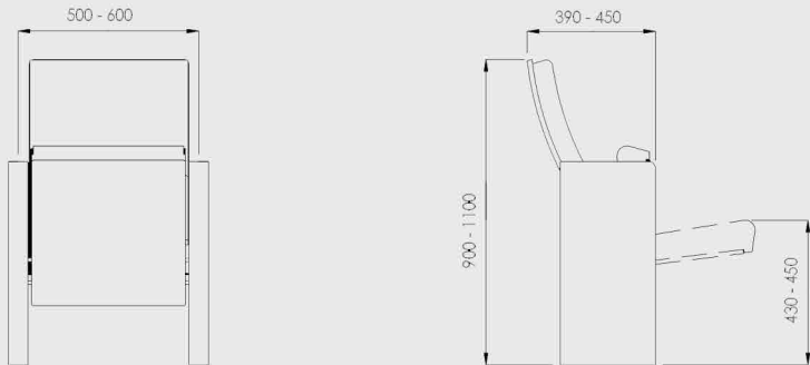
A) standard version
