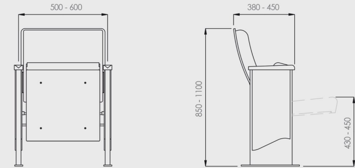
C/ steel version
