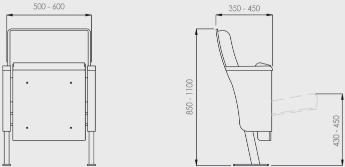
A) standard version
